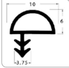
AK 100 Kapı Fitili - Oval Yandan / Door Wick - Oval Sideways
