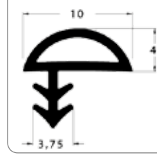
AK 110 Kapı Fitili - Oval Yandan / Door Wick - Oval Sideways
