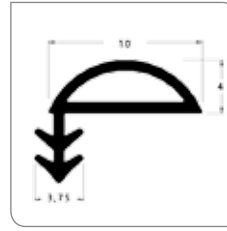
AK 010 Kapı Fitili - Oval Yandan / Door Wick - Oval Sideways
