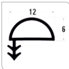
AK 002 Kapı Fitili - Oval Yandan / Door Wick - Oval Sideways
