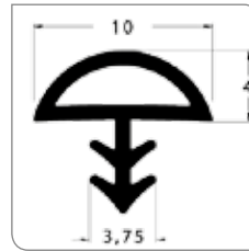
AK 210 Kapı Fitili - Oval Ortadan / Door Wick - Oval Sideways
